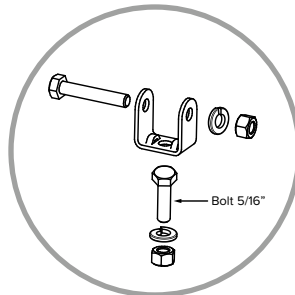
U-Bracket
