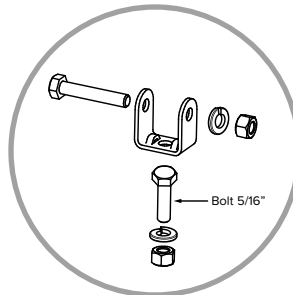
U-Bracket
